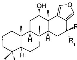
Figure 2. Computer-generated X-ray crystal structure of sesterstatin 5 ( 1b ) and methanol solvate
